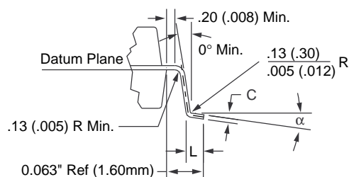
Lead Detail
